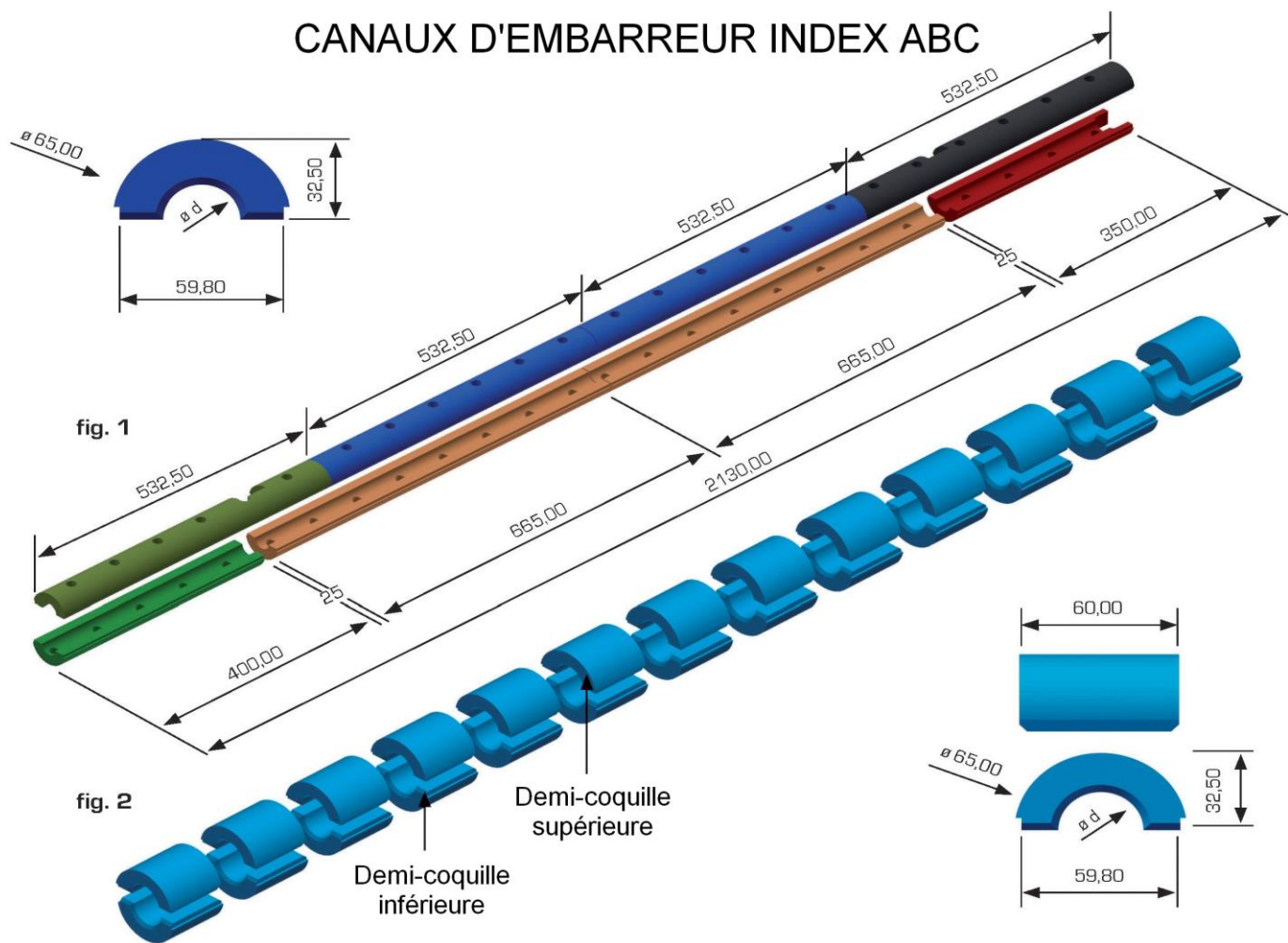
fig 1: Solution Unilock fig 2 : Montage standard
